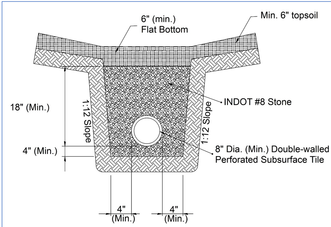
FIGURE 4-3 Bedding and Backfill for Sub-drains under Swales
